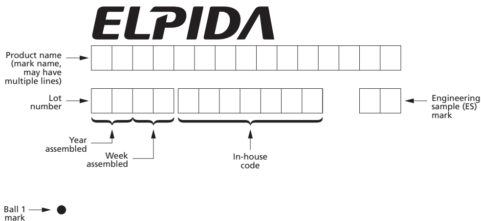
Figure 3: Legacy BGA Component with Elpida Part Mark
