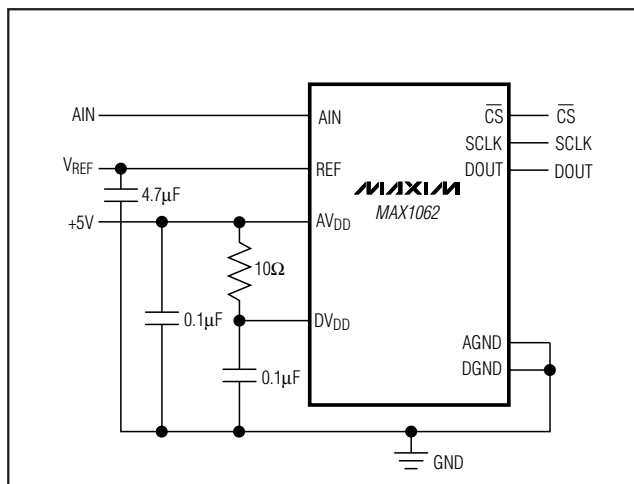
Figure 14. Powering \text{AV}_{\text{DD}} and \text{DV}_{\text{DD}} from a Single Supply
